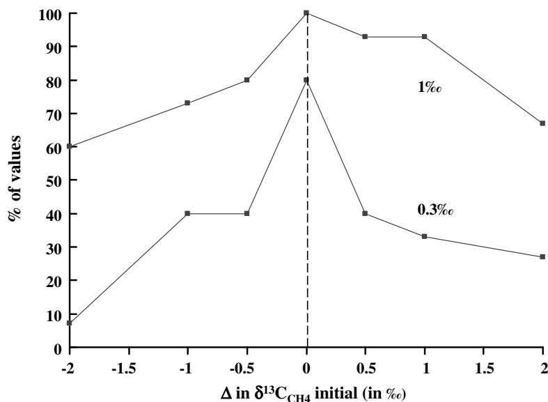
Fig. 8. Sensitivity of the model calculated values to changes in initial value parameter \delta^{13}\text{C}_{\text{CH}_4} for methane. When \delta^{13}\text{C}_{\text{CH}_4} is equal to the measured value ( \Delta = 0 ), 100% of model calculated \delta^{13}\text{C} values for C2, C3 and n -C4 for all samples are within 1‰ of the measured values ( \delta^{13}\text{C}_{\text{calculated}} - \delta^{13}\text{C}_{\text{measured}} < 1\text{‰} ) (see text). If \Delta changes by as little as 0.5–1‰ in the direction of either more ^{13}\text{C} -enrichment or ^{13}\text{C} -depletion as would be the case if the primary methane isotope value was affected by mixing of gases from different sources or secondary fractionation processes, the percentage of calculated values which are in agreement with the measured values decreases significantly.
