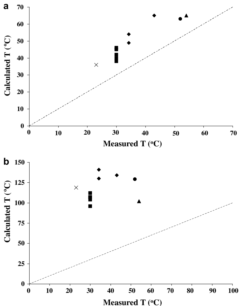
Fig. 5. Measured groundwater temperatures ( ^{\circ}\text{C} ) for Kidd Creek samples (squares); Copper Cliff South (crosses); Dreifontein (diamonds) Mponeng (circles) and Kloof (triangles) versus temperatures calculated based on hydrogen isotope geothermometers for (a) \text{H}_2\text{O}_{(l)}\text{-H}_{2(g)} and (b) \text{CH}_4\text{-H}_2 from Horibe and Craig (1995). All calculated temperatures are significantly higher than measured groundwater temperatures indicating the \text{H}_2\text{O-H}_2\text{-CH}_4 system is not at isotopic equilibrium. Data from Kidd Creek show a vertical distribution because all groundwaters have approximately the same measured temperature.
